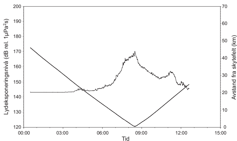
Figur 3.4.2. Som Figur 3.4.1, men denne figuren viser beregnet lydeksponeringsnivå. (As Figure 3.4.1, but this figure shows estimated sound exposure level.)
